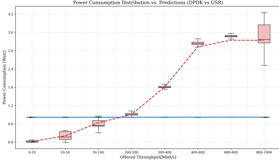
Figure 4: Process-attributed power-consumption distributions and MLP profiling-model predictions for the DPDK (blue, solid) and USR (red, dashed) realizations as a function of offered throughput. Box plots show empirical variability across profiling runs.
