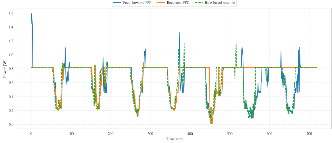
Figure 6: Interval-averaged attributed power P_i over the test horizon for the evaluated controllers.
