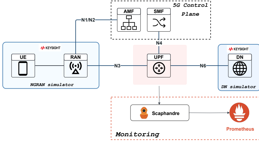
Figure 2: Physical testbed architecture used for UPF profiling and metric collection. The Keysight LoadCore platform simulates UE/RAN (N3) and data-network (N6) endpoints. The 5G control plane (AMF, SMF) manages sessions via N4. Scaphandre monitors power attributed to the UPF processes via RAPL-derived estimates and exports metrics to Prometheus.
