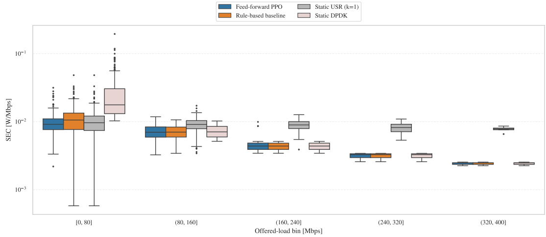
Figure 7: Specific energy consumption SEC_i by offered-load bins.
