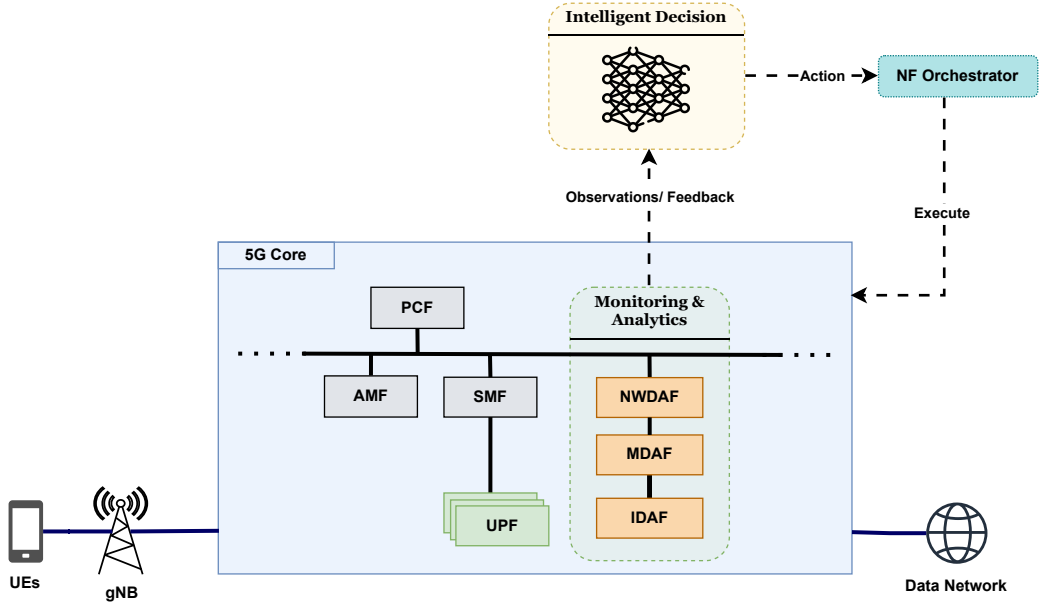
Figure 1: Target online closed-loop UPF orchestration architecture. The present paper validates the decision logic offline in a measurement-grounded digital twin before any live deployment.
